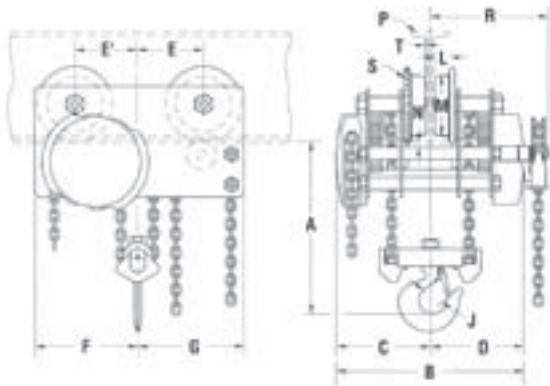
PLAIN & GEARED
